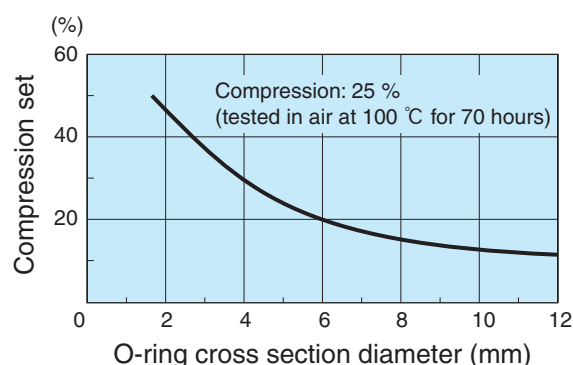
Fig. 2.3.1 Relation between O-ring cross section diameter and compression set
