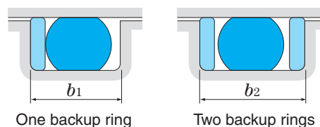
Groove dimensions for static sealing on cylindrical surface
