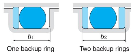
Groove dimensions for dynamic sealing and static sealing on cylindrical surface
