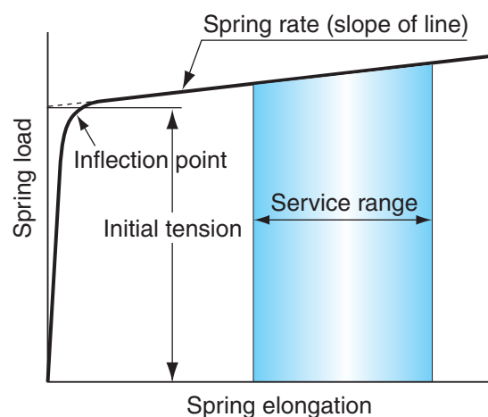
Fig. 1.1.2 Spring properties for seal
