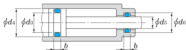
Groove dimensions for dynamic sealing and static sealing on cylindrical surface
