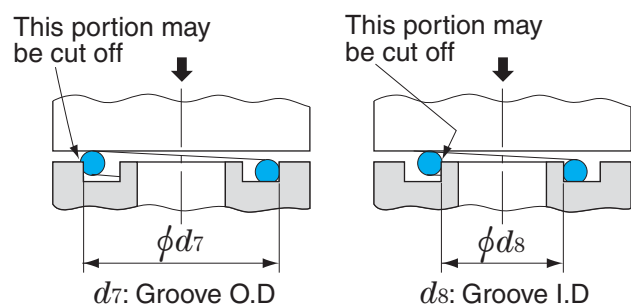
Fig. 2.4.5 O-ring protrusion
